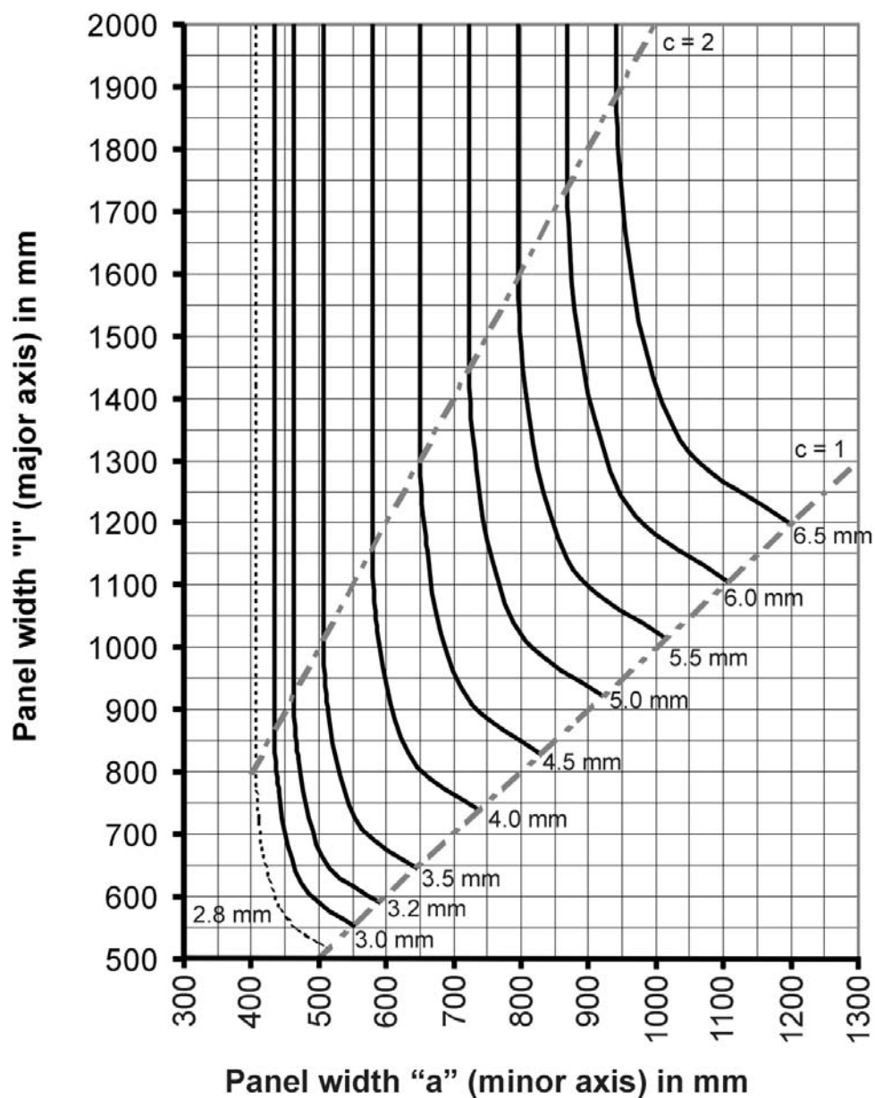
Figure 10 — Minimum thickness of fuel tanks plated in carbon steel for heads not exceeding 2.5 m
