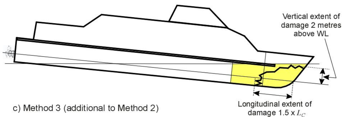
Figure 6 — Methods for establishing the location of the collision bulkhead
