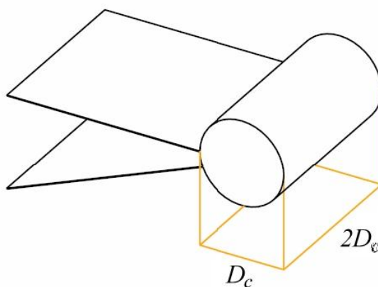
Figure 12 — Assumed panel dimensions for determining the design pressure P
